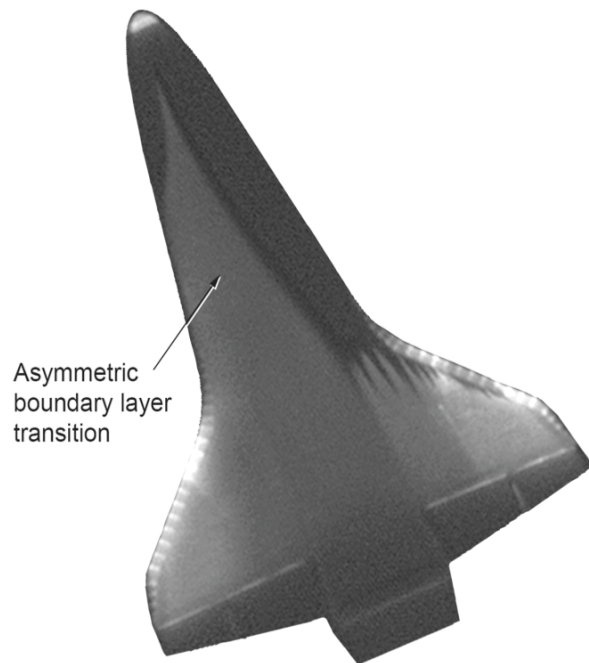
Figure 3: Thermal image of Endeavour during STS-134 re-entry near the point of closest approach, Mach 5.8, AOA = 28.8 deg, Slant Range ~32 nautical miles.
