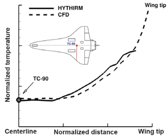
Figure 9: Comparison of Mach 8.4 Surface Temperature Distribution and Fully Turbulent CFD.
