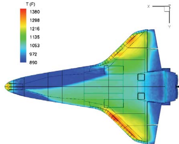
Figure 7b: STS-134 3-D temperature mapping. Mach = 5.8, AOA = 28.8 deg
