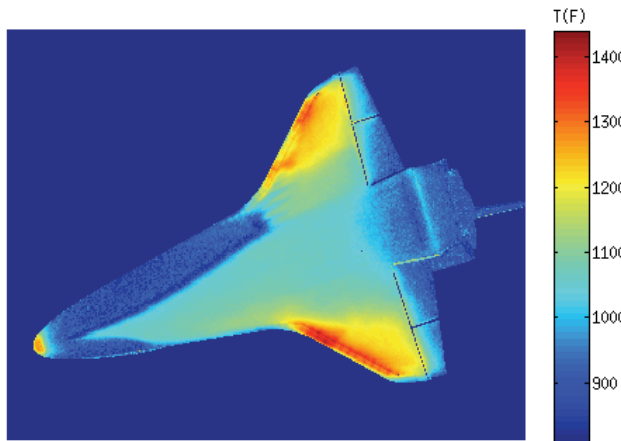
Figure 7a: STS-134 2-D temperature mapping. Mach = 5.8, AOA = 28.8 deg
