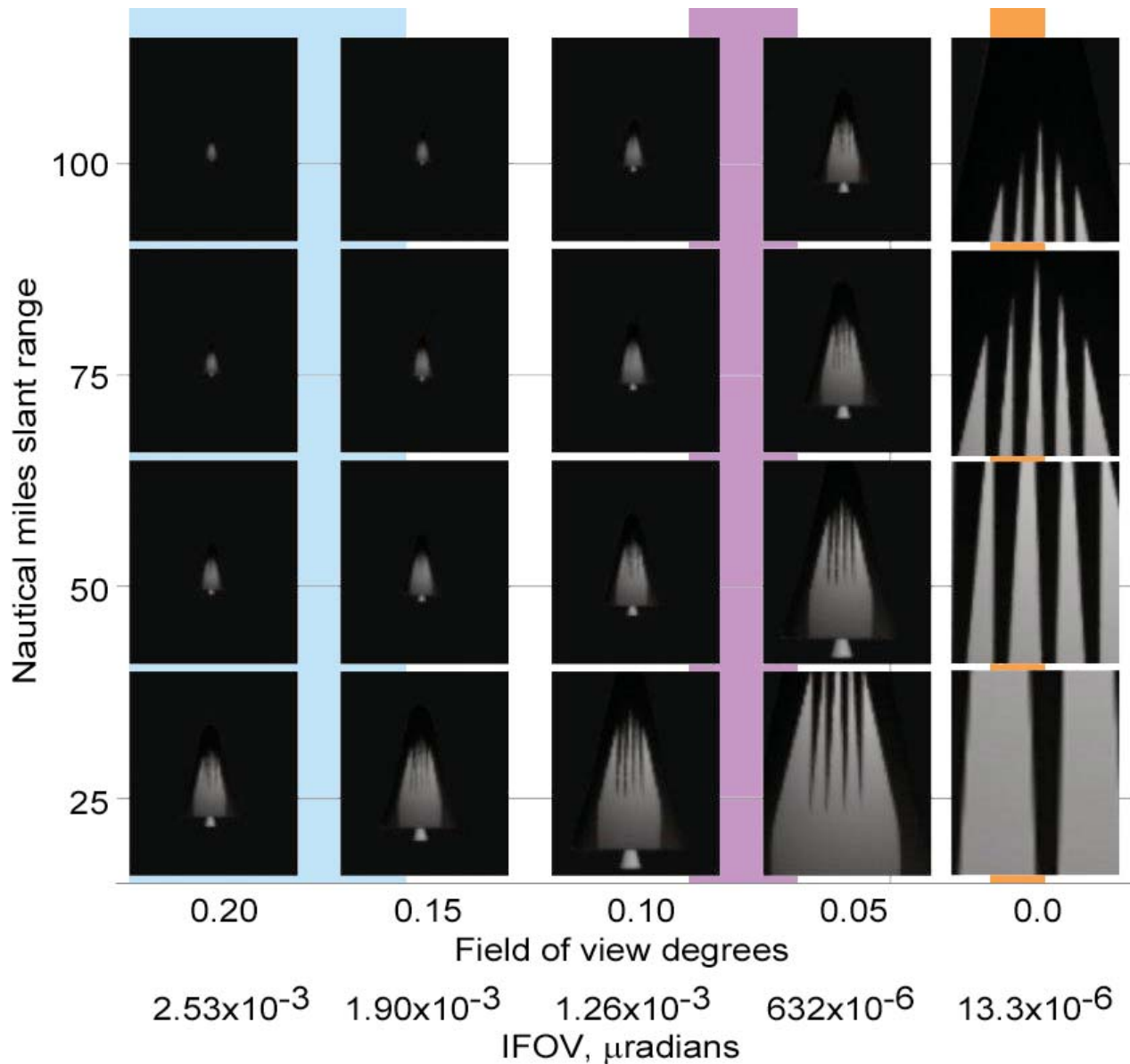
Figure 13: Synthetic images of expected spatial resolution as a function of IFOV and slant range. Blue - capability used by HYTHIRM; Magenta – emerging commercial capability; Tan – existing large aperture (fixed location) ground-based imaging system.
