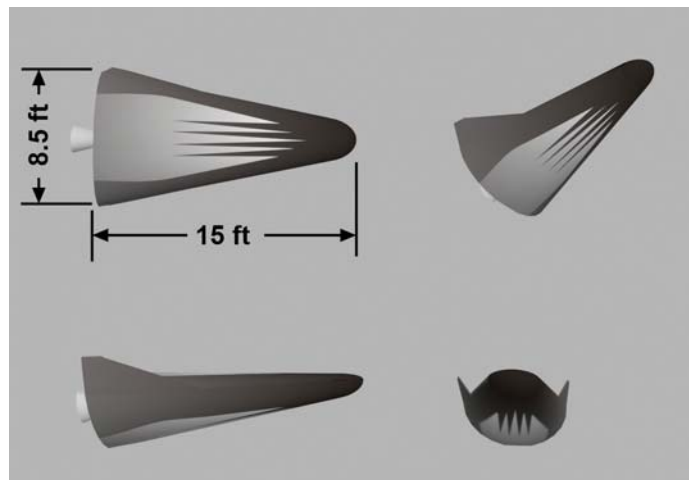
Figure 12: Notional hypersonic flight test vehicle with features mimicking thermal patterns on the lower surface.
