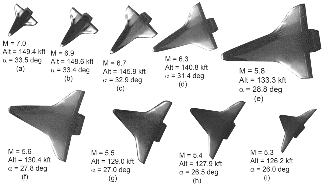
Figure 2: Time sequence of near infrared intensity images showing the evolution of hypersonic boundary layer transition on Shuttle Endeavour’s lower surface during STS-134 re-entry. Total elapsed time ~ 2 minutes. Elevated temperatures are shown in lighter gray
