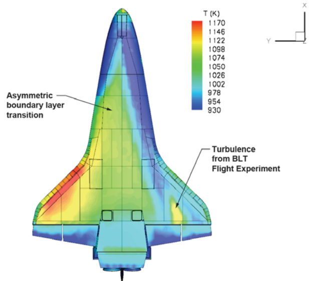
Figure 11: Thermal mapping of STS-119 asymmetric boundary layer transition (ABL). Mach 8.4.
