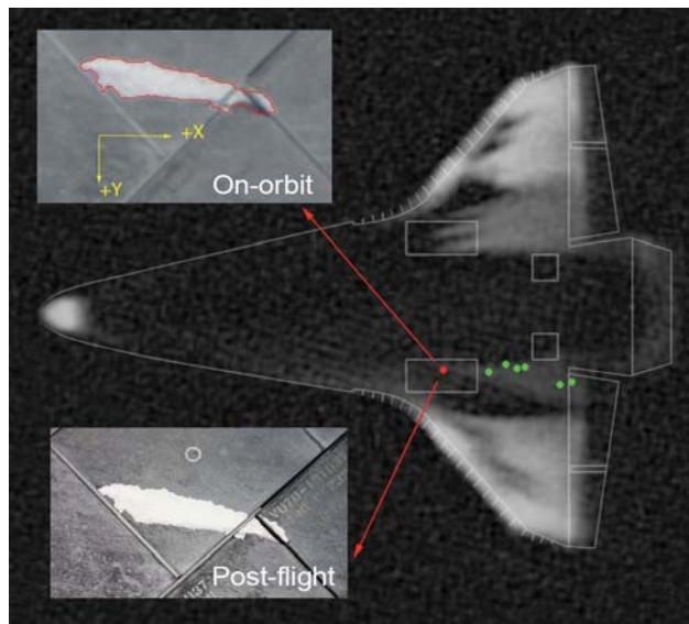
Figure 5: Boundary layer transition induced by a tile cavity. STS-134, Mach = 6.9, AOA = 33.4 deg.
