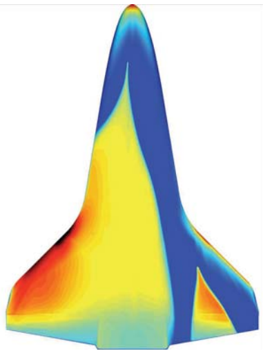
Figure 10: Predicted turbulent spreading from a point source (Ref. 43). Temperature scale on Fig. 11 applies.
