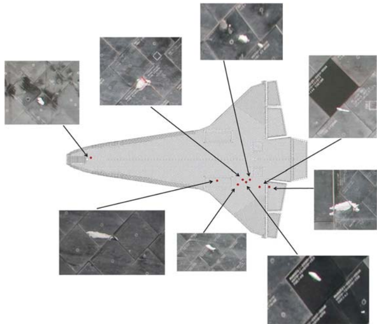
Figure 4: STS-134 tile impact damage observed on orbit as Endeavour approached the space station.
