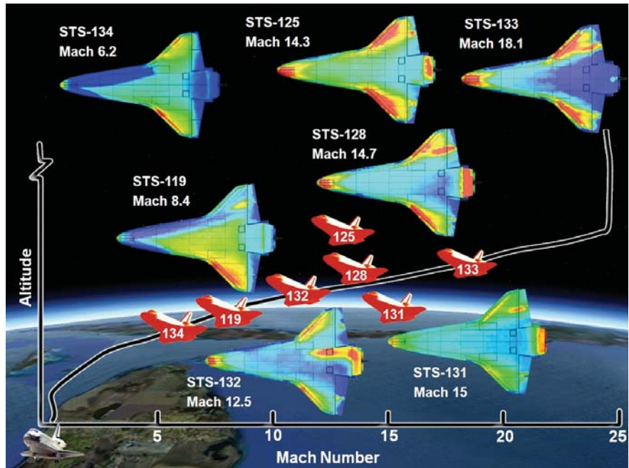
Figure 1: HYTHIRM Shuttle thermal imaging Mach envelope. (color pallet varied to enhance detail on each flight)
