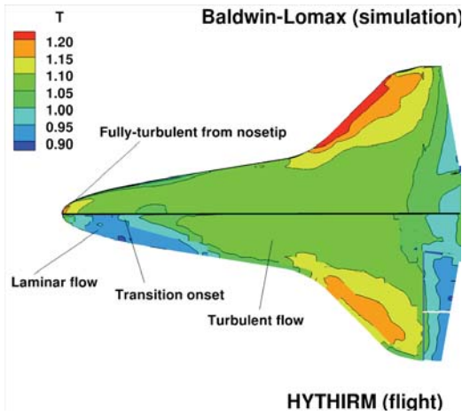
Figure 8: Comparison of Mach 8.4 Fully Turbulent CFD with STS-119 Thermal 3-D Mapping.
